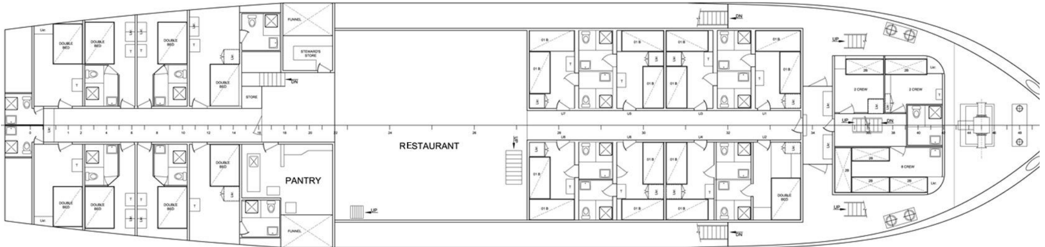
UPPER DECK PLAN
