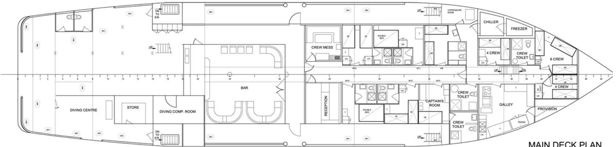
MAIN DECK PLAN
